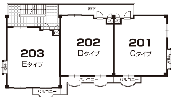
●2階平面図
