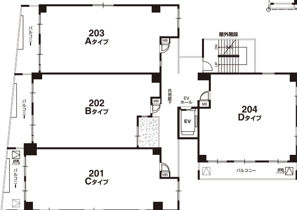
●2階平面図
